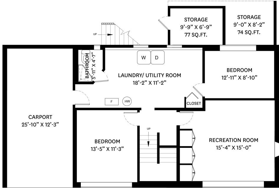
LOWER FLOOR PLAN Ceiling Height: 7'-9"
